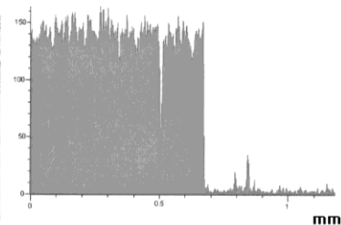
Copper Ka1
